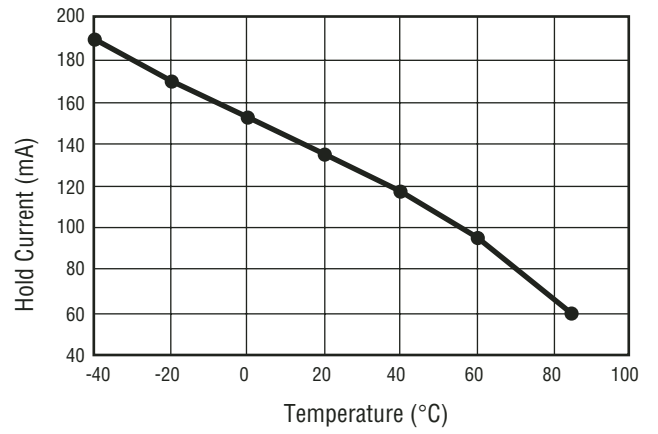
Hold Current vs Temperature
